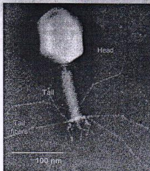
Figure 1: Electron micrograph of a bacteriophage
