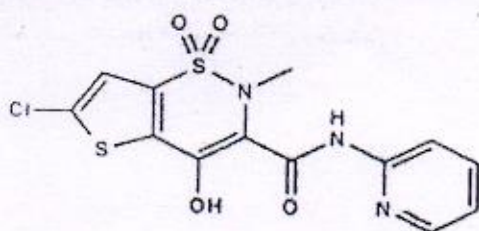
Figure 1: Chemical structure of lornoxicam
