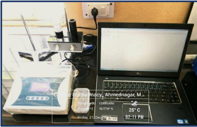
Digital Plethysmometer
